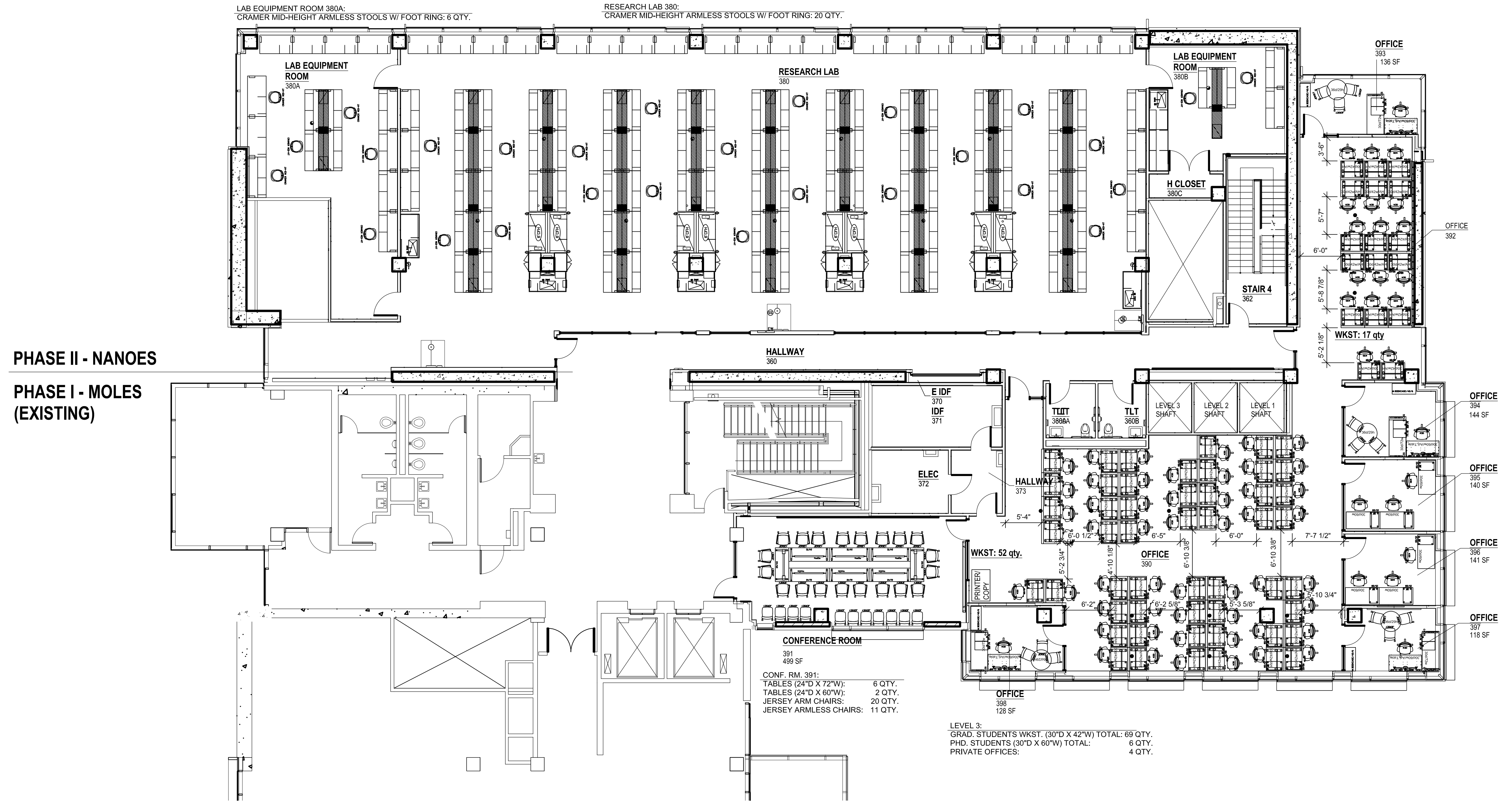
FURNITURE (30"d X 42"w) PLAN - LEVEL THREE UW NANO TECHNOLOGY SCALE: 1/8" = 1'-0"
